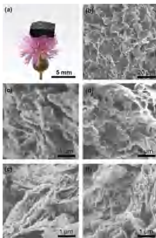
Figure 2. Morphology of the 3D GF during Li deposition and dissolution. (a) Side-view optical image of bulk GF on a flower. (b) SEM image of GF with large pores between the graphene sheets. (c–f) Morphology of the SCG anode during the lithiation and delithiation process: (c) first and (e) 10 th deposition; (d) first and (f) 10 th dissolution.
