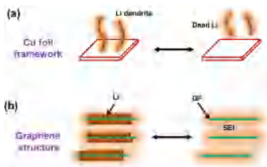
Figure 1. Schematic diagrams of a Li metal anode with different structures during Li deposition and dissolution. (a) Without a graphene framework, Li dendrites appear during Li deposition, thus leading to a large amount of dead Li during Li dissolution. (b) The SCG-structured anode depicts a stable and uniform Li deposition and dissolution with high efficiency and low resistance.
