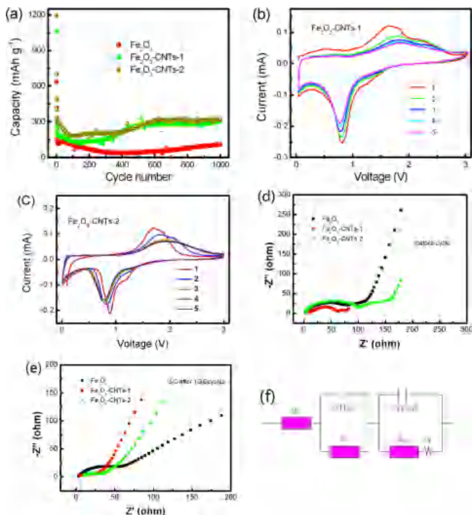
Figure 4. (a) Long-term cycling performance of samples at a high current density of 5 C, cyclic voltammogram profiles of network (b) \alpha - \text{Fe}_2\text{O}_3 -CNTs-1 composite, and (c) \alpha - \text{Fe}_2\text{O}_3 -CNTs-2 composite, EIS spectra of samples (d) before cycling and (e) after 1000 cycles at the current density of 5 C, and (f) an electrochemical equivalent circuit.
