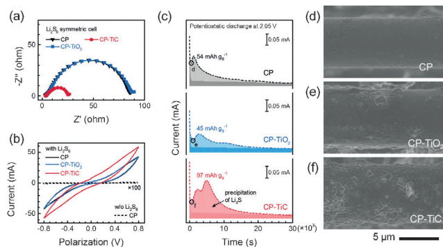
Figure 2. Electrochemical kinetics. a) EIS and b) CV of \text{Li}_2\text{S}_6 symmetric cells employing CP, CP- \text{TiO}_2 , and CP-TiC as current collectors. c) Potentiostatic discharge curves of a \text{Li}_2\text{S}_8 /tetraglyme solution at 2.05 \text{ V} on different surfaces. The scale of the y-axis is indicated by the bar in the right. The lighter color indicates the precipitation of \text{Li}_2\text{S} , whereas the darker color represents the reduction of \text{Li}_2\text{S}_8/\text{Li}_2\text{S}_6 . The capacity of \text{Li}_2\text{S} deposition is indicated over each curve. d–f) SEM images of the initial nucleation of \text{Li}_2\text{S} on different surfaces as indicated in (c). The scale bar is at the bottom right.
