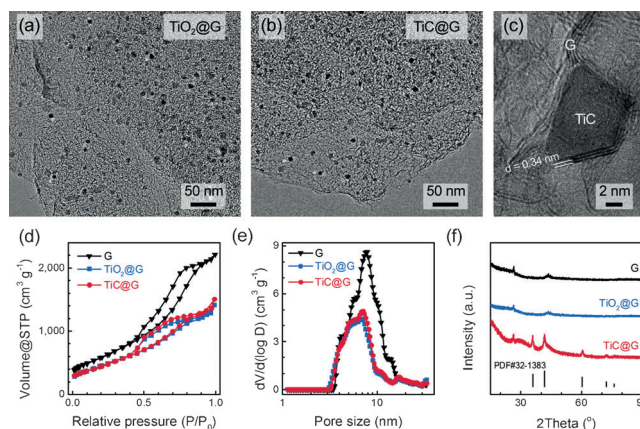
Figure 3. Structural characterization. Transition electron microscopy (TEM) images of a) \text{TiO}_2\text{@G} and b) \text{TiC@G} . High-resolution TEM image of c) \text{TiC@G} . d) \text{N}_2 isotherms and e) corresponding pore-size distribution based on density functional theory. f) XRD patterns.
