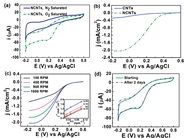
Figure 3. (a) Cyclic voltammograms of the NCNTs at a scan rate of 50 mV/s in 0.5 M H 2 SO 4 solution saturated with N 2 or O 2 . (b) Rotating-disk-electrode (RDE) linear sweep voltammograms of the NCNTs and undoped CNTs in oxygen-saturated 0.5 M H 2 SO 4 at a scan rate of 10 mV/s. (c) RDE curves of the NCNT in oxygen-saturated 0.5 M H 2 SO 4 with different speeds of 100, 400, 900, and 1600 rpm at a scan rate of 10 mV/s (the inset showing the Koutecky–Levich plots of the NCNT derived from RDE measurements). (d) Electrochemical stability measurements of the NCNT by using continuous cyclic voltammetry in oxygen-saturated 0.5 M H 2 SO 4 at a scan rate of 50 mV/s.
