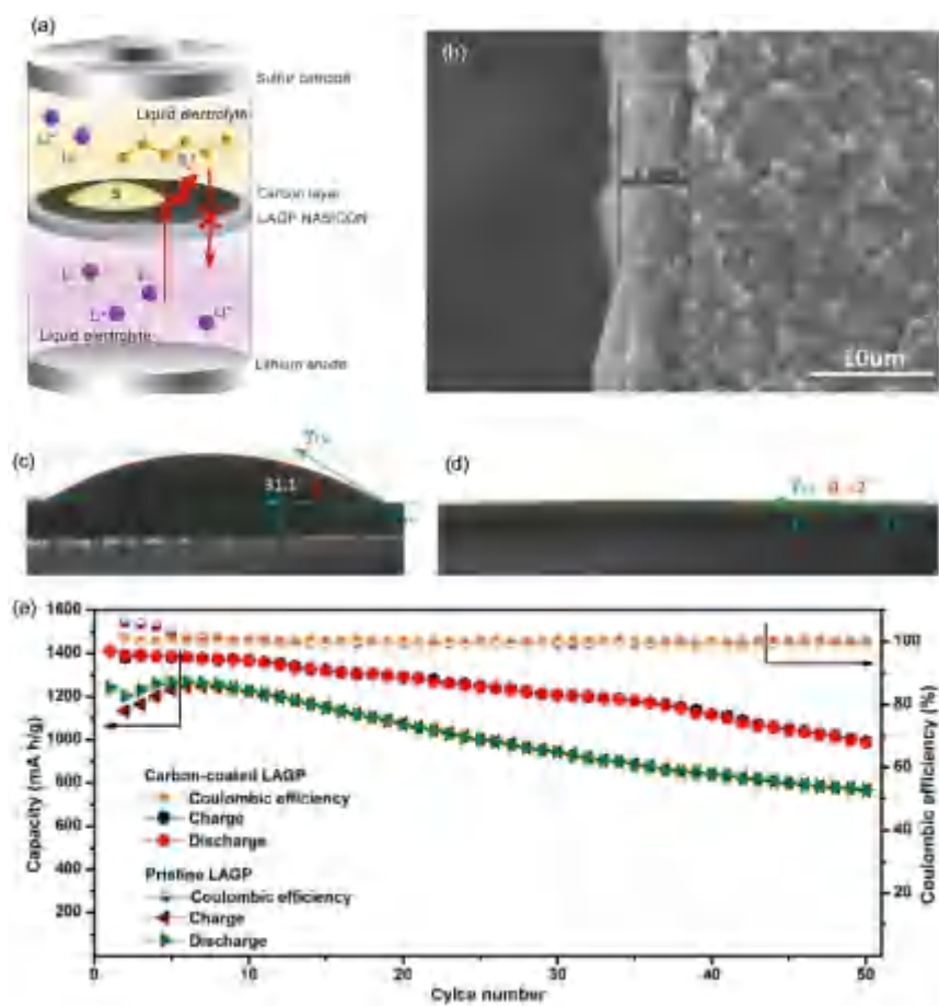
Figure 12 Li-S battery configuration with a carbon-coated LAGP electrolyte. (a) Schematic illustration. (b) SEM image of the cross section of the carbon-coated LAGP. Contact angle snapshots for Li 2 S 2 /tetraethyleneglycol dimethylether (TEGDME) on (c) pristine LAGP and (d) carbon-coated LAGP. (e) Cycling performance of the Li-S cells. Reprinted with permission from Ref. [150], copyright 2017, Elsevier (color online).
