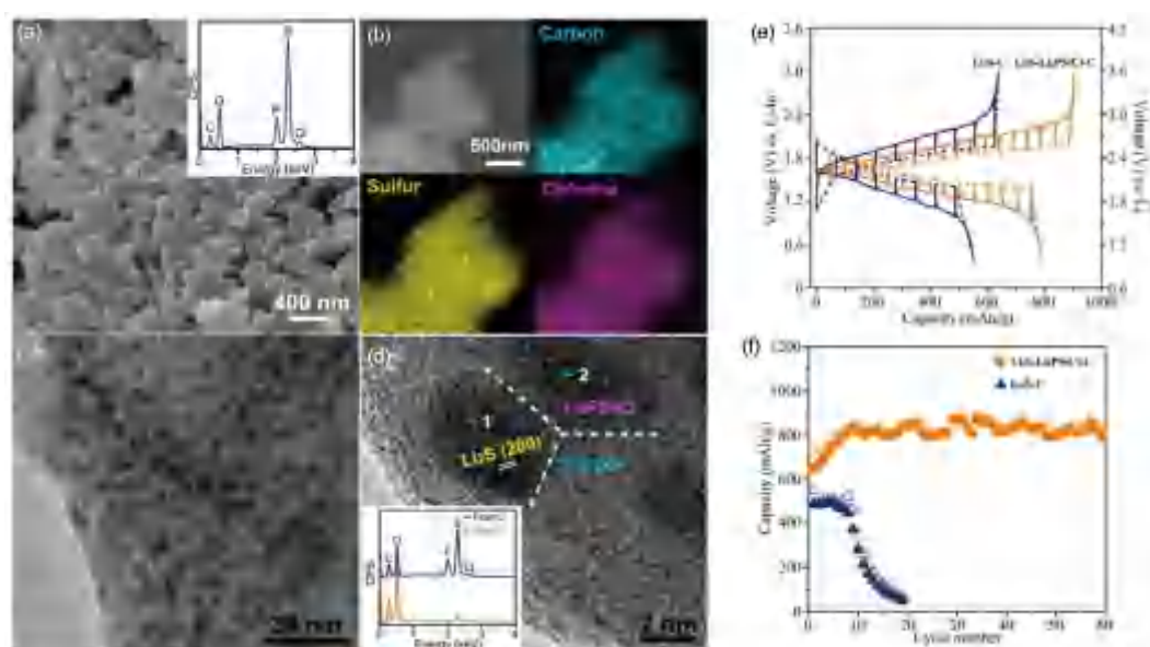
Figure 3 \text{Li}_2\text{S-Li}_6\text{PS}_5\text{Cl-C} electrode. (a) Scanning electron microscopy (SEM) image of the \text{Li}_2\text{S-Li}_6\text{PS}_5\text{Cl-C} nanocomposite. The inset shows the energy-dispersive X-ray spectroscopy (EDS) result. (b) The elemental mappings of carbon, sulfur, and chlorine in the composite. (c) The TEM image of the \text{Li}_2\text{S-Li}_6\text{PS}_5\text{Cl-C} nanocomposite. (d) The high-resolution TEM image of the \text{Li}_2\text{S-Li}_6\text{PS}_5\text{Cl-C} nanocomposite, and the inset shows the EDS results at point 1 and point 2, respectively. (e) Equilibrium (open-circuit) voltage (dashed lines) and transient voltage (solid lines) profiles versus capacity for the 1st cycle of the \text{Li}_2\text{S-C} and \text{Li}_2\text{S-Li}_6\text{PS}_5\text{Cl-C} nanocomposite electrodes. (f) Cycling performances of the \text{Li}_2\text{S-C} and \text{Li}_2\text{S-Li}_6\text{PS}_5\text{Cl-C} nanocomposite electrodes at 50 \text{ mA g}^{-1} . Reprinted with permission from Ref. [80], copyright 2016, American Chemical Society (color online).
