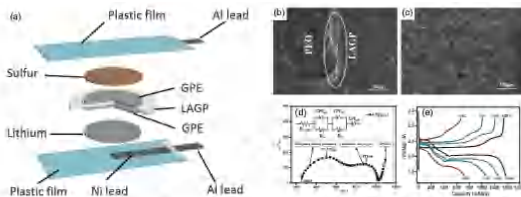
Figure 10 Li-S cell with gel-ceramic multi-layer electrolyte. (a) Schematic illustration; (b) SEM image of the cross section of the gel-ceramic multi-layer electrolyte; (c) SEM image of porous carbon paper soaked with the gel-polymer electrolyte; (d) Nyquist plot of the Li-S cell at the fully charged state and the inset shows the proposed equivalent circuit for the Li-S cell; (e) initial discharge/charge profiles at C/20, C/10, C/5 and C/2 rates. Reprinted with permission from Ref. [141], copyright 2016, Royal Society of Chemistry (color online).
