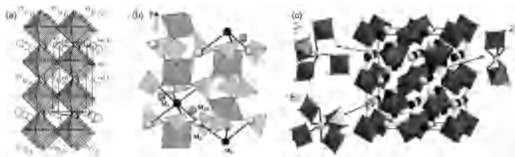
Figure 8 (a) Crystal structure of \text{Li}_{1-x}\text{La}_{2/3-x}\square_{1/3-2x}\text{TiO}_3 ( \bigcirc =La, Li or vacancies in position (0, 0, 0) ; \bigcirc =La, Li or vacancies in position (0, 0, \frac{1}{2}) ; lines represent the unit cell). Reprinted with permission from Ref. [120], copyright 1996, Elsevier. (b) Rhombohedral structure of NASICON materials in which M_1 , M_{1/2} , and M_2 sites are susceptible to be occupied by lithium. Reprinted with permission from Ref. [126], copyright 2005, American Physical Society. (c) The crystal structure of a conventional garnet \text{A}_3\text{B}_3\text{C}_2\text{O}_{12} where octahedra indicate \text{CO}_6 units and black and grey spheres represent A and B cations respectively. In addition to the three C sites occupied in conventional garnets, suitable sites for lithium cations in \text{Li}_5\text{La}_3\text{M}_2\text{O}_{12} include the six octahedral and two trigonal prismatic sites indicated. 18 selected positions for these two additional coordination sites are indicated by transparent spheres within the garnet unit cell. Reprinted with permission from Ref. [132], copyright 2010, Royal Society of Chemistry.
